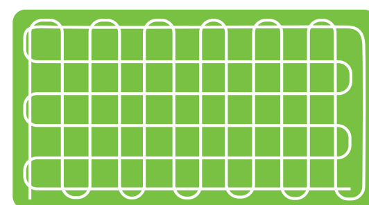
CRISS-CROSS APPLICATION
